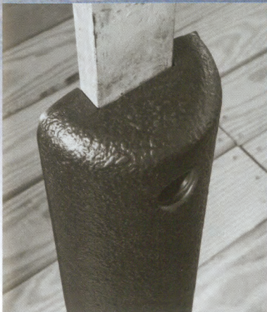
4 inch bumper w/ 0.625 x 3 inch wide groove nominal
